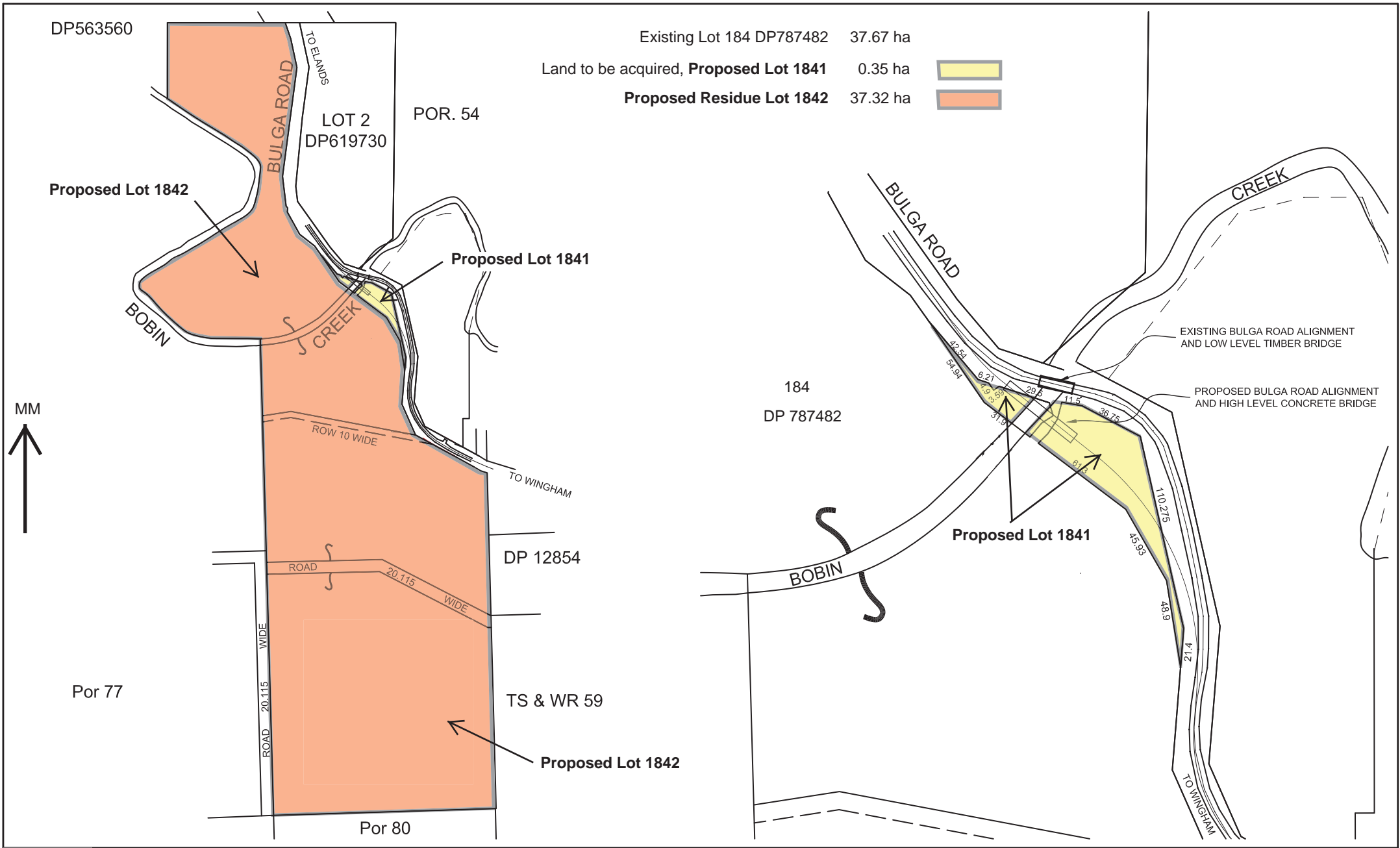
REPLACEMENT OF TIMBER BRIDGE ON BULGA ROAD PLAN SHOWING PROPOSED ROAD WIDENING AND LAND ACQUISITION
